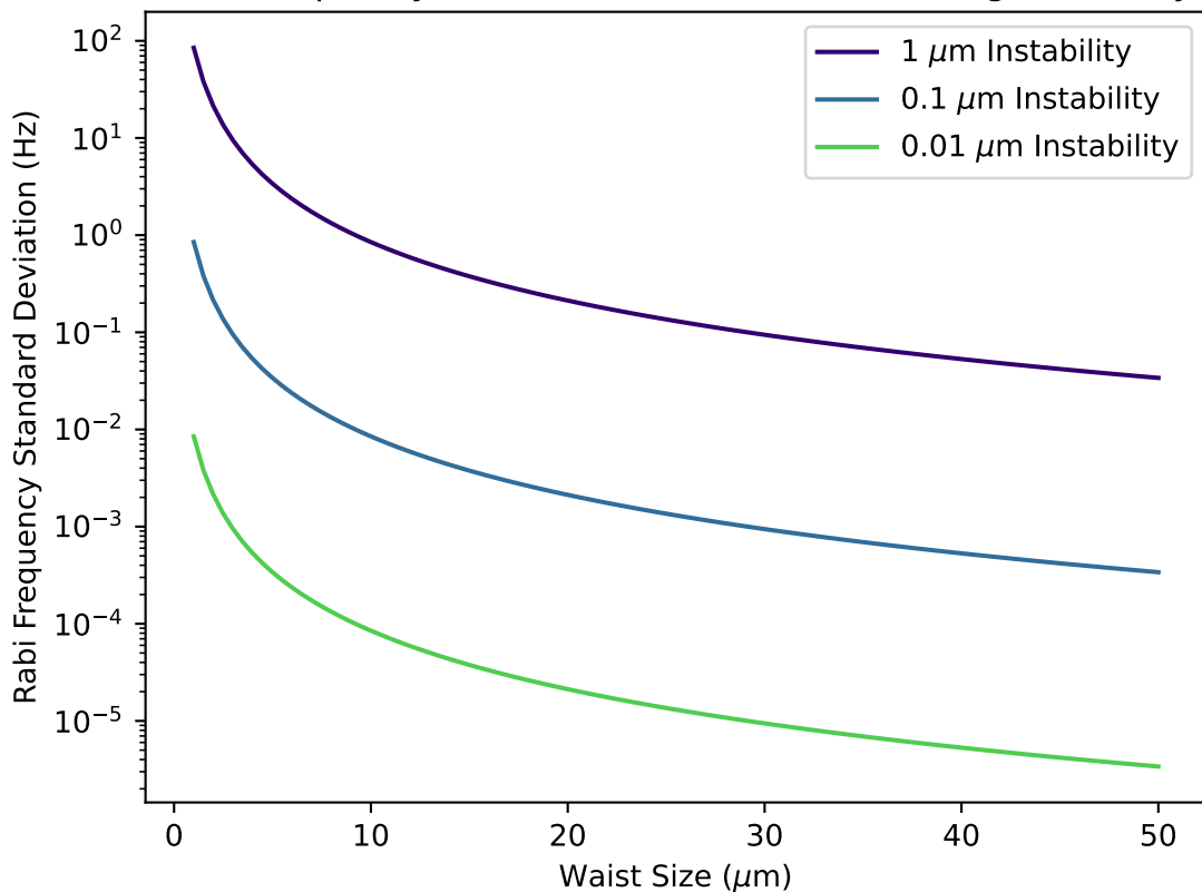
Rabi Frequency Deviation Due to Laser Pointing Instability
